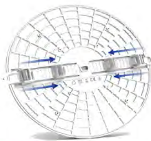
FRAMELESS DESIGN 01 ADJUSTABLE Fit cut-out from 70-205mm
